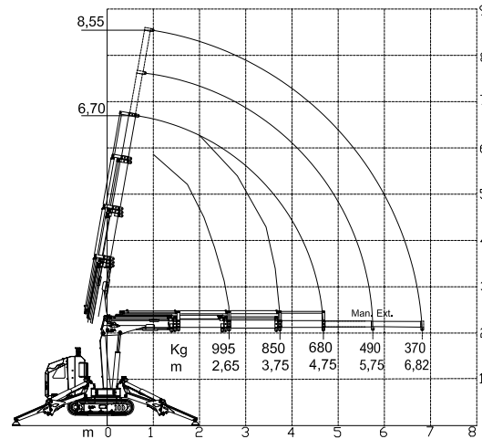
MCR30 load chart
