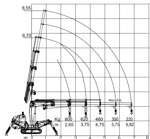
MCR30 narrow stabilization + winch 800kg load chart
