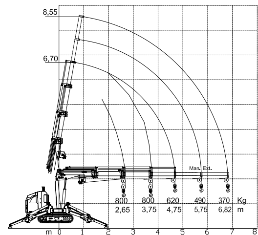
MCR30 + winch 800kg load chart
