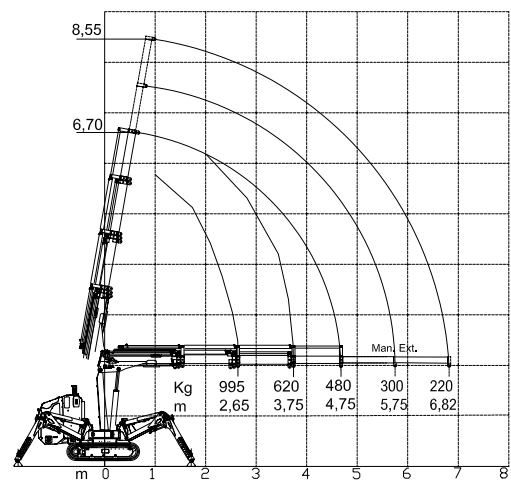
MCR30 narrow stabilization load chart
