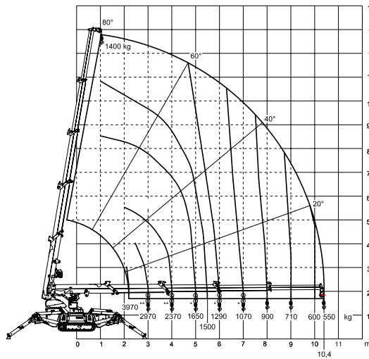
MCX110 + winch load chart
