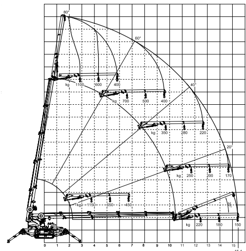
MCX110 + jib + winch load chart
