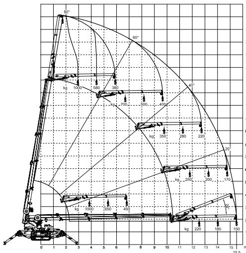
MCX110 + jib + hook load chart
