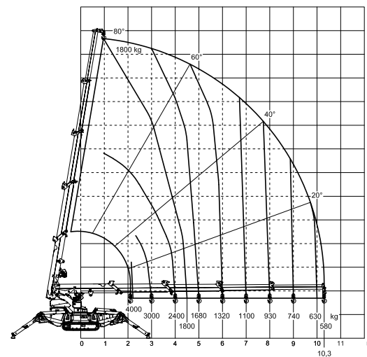
MCX110 + hook load chart
