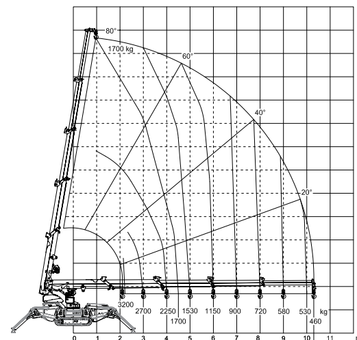
MCX90 + hook load chart
