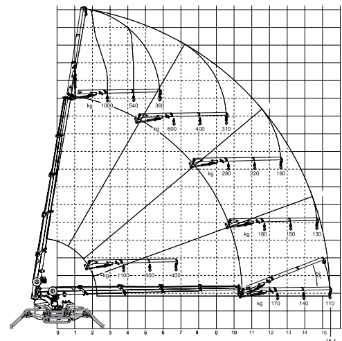
MCX90 + jib + winch load chart
