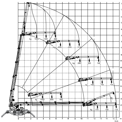
MCX90 + jib + hook load chart
