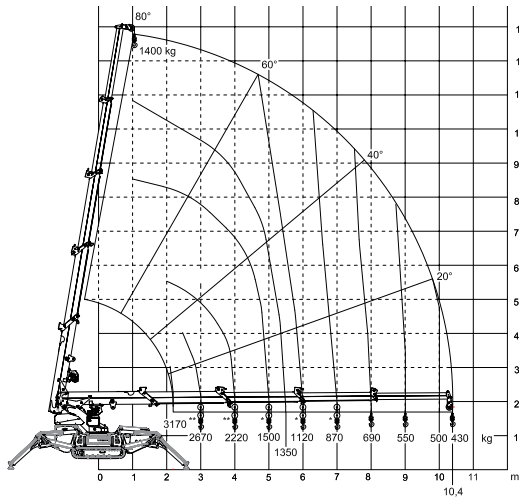
MCX90 + winch load chart
