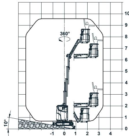
Working diagram on stabilizers
