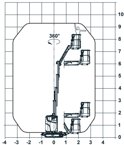
Working diagram on crawlers
