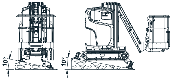
Max. tilt for selfstabilizers
